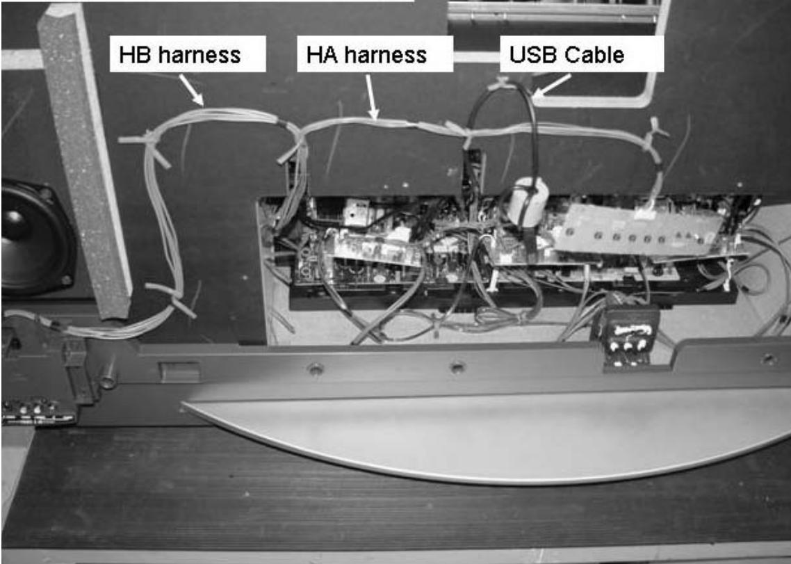
KDP-51/57WS655 front wire dressing
