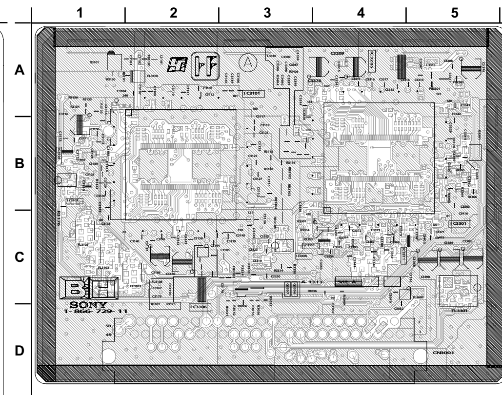
BH [A/D, HELIOS] (PN A-1111-561-A) COMPONENT SIDE
