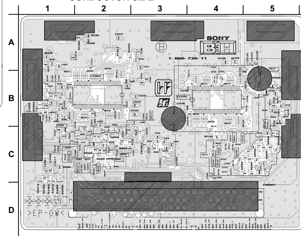
BH [A/D, HELIOS] (PN A-1111-561-A) CONDUCTOR SIDE
